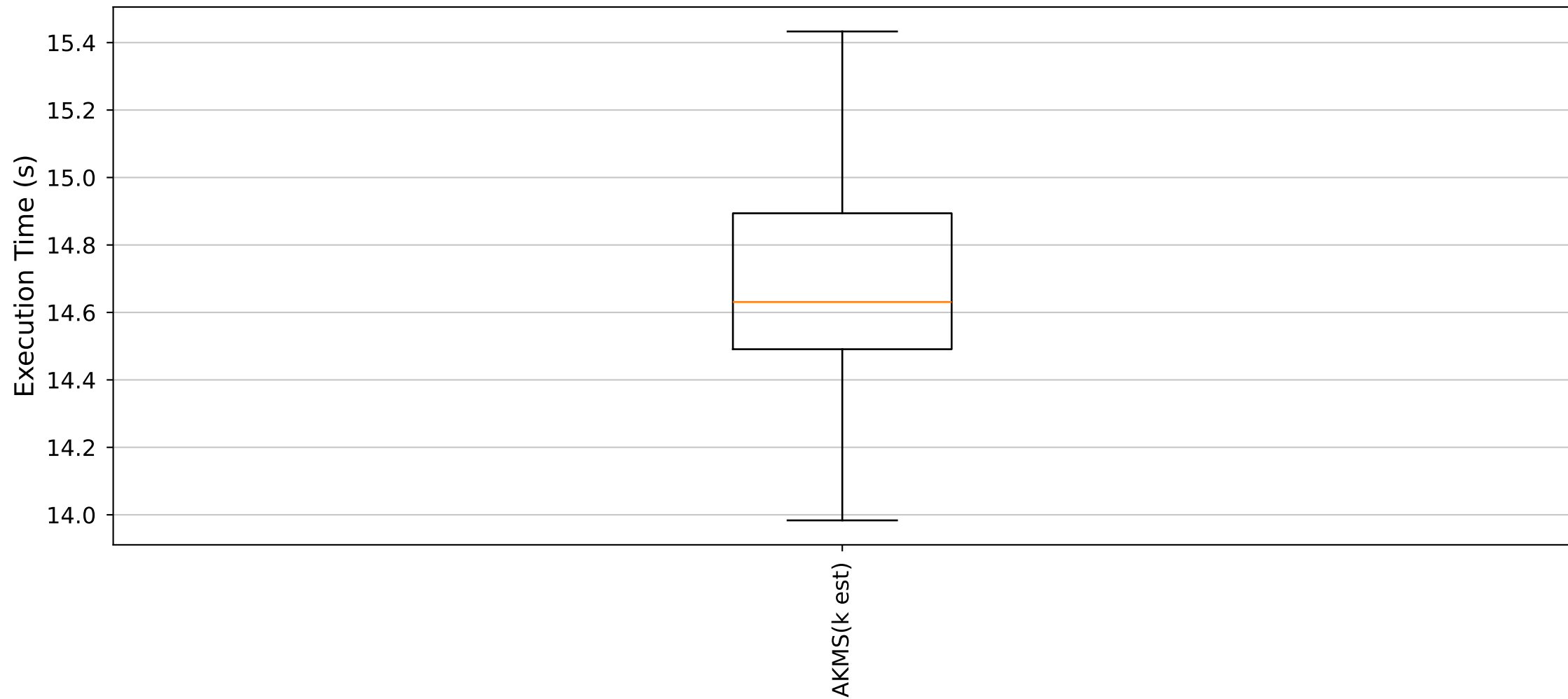
YARA Rules Execution Time Distribution (Cluster2_Size100 dataset)
